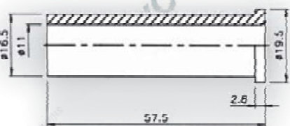
RUBBER TUBE FOR PLS-28-PM
