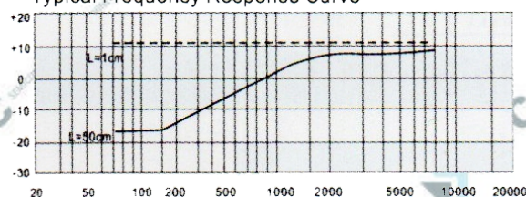
Typical Frequency Response Curve
