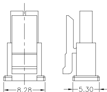
(2PIN Circuit Housing)
