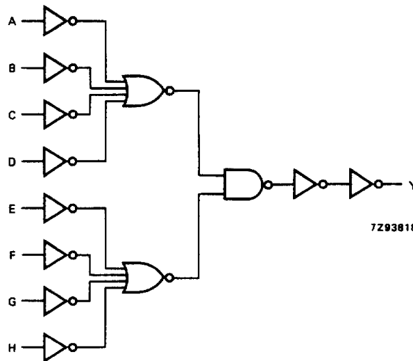
Fig.5 Logic diagram.
