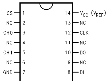
ADC0832 2-Channel MUX Small Outline Package (WM)
