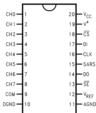
ADC0838 8-Channel Mux Small Outline/Dual-In-Line Package (WM and N)
