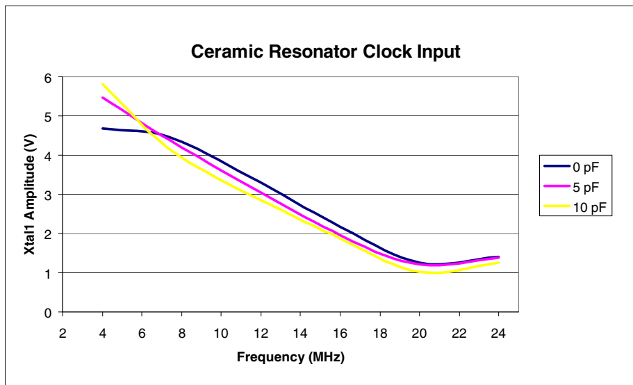
Figure 16-3. Ceramic Resonator Clock Source
