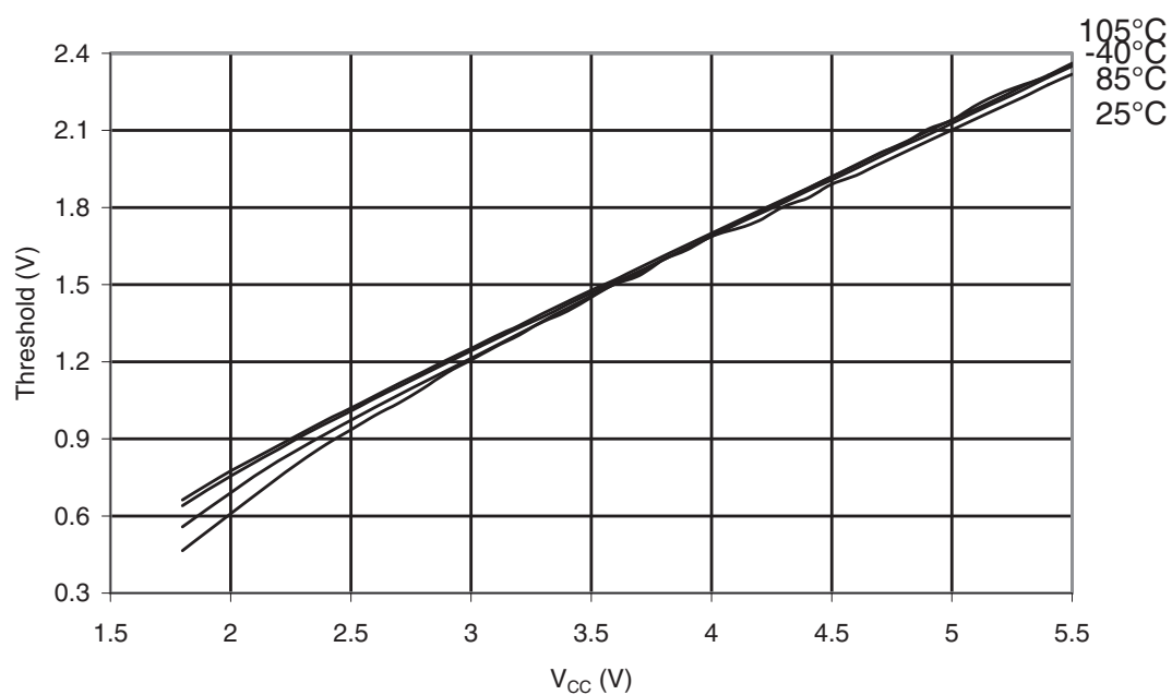
Figure 32-25. ATmega48PA: I/O Pin Input Threshold Voltage vs. V_{CC} ( V_{IL} , I/O Pin read as '0')
