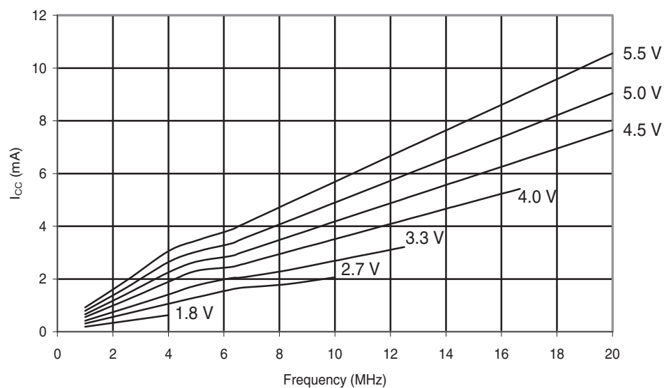
Figure 31-191. ATmega168A: Active Supply Current vs. Frequency (1-20MHz)
