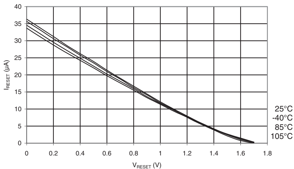
Figure 31-349. ATmega328P: Reset Pull-up Resistor Current vs. Reset Pin Voltage ( V_{CC} = 1.8V )
