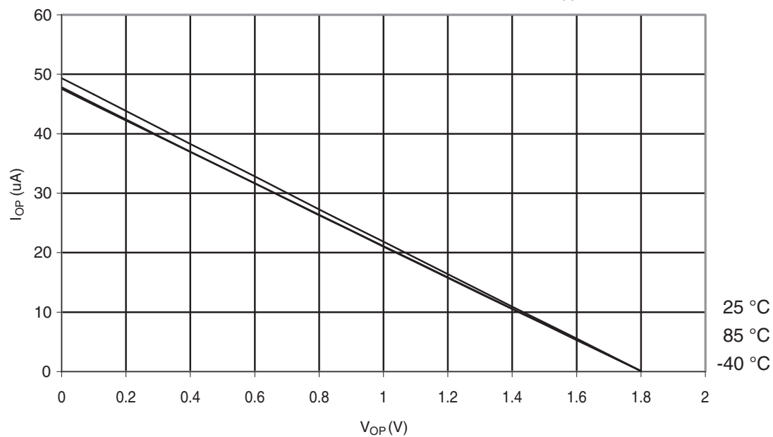
Figure 31-299. ATmega328: I/O Pin Pull-up Resistor Current vs. Input Voltage ( V_{CC} = 1.8\text{ V} )
