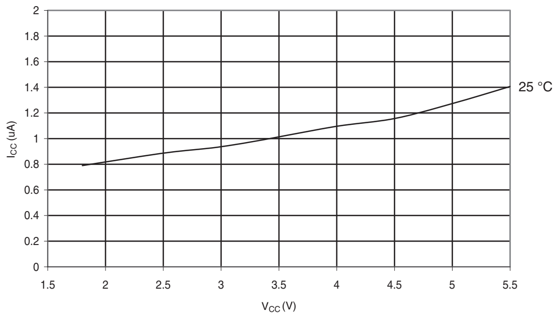
Figure 31-297. ATmega328: Power-Save Supply Current vs. V_{CC} (Watchdog Timer Disabled and 32kHz Crystal Oscillator Running)
