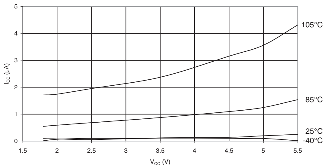
Figure 31-152. ATmega88PA: Power-Down Supply Current vs. V_{CC} (Watchdog Timer Disabled)
