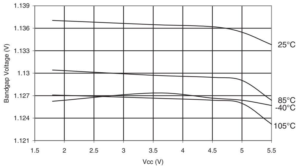
Figure 35-34. ATmega328P: Calibrated Bandgap Voltage vs. V CC
