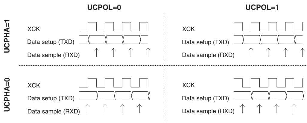
Figure 21-1. UCPHA n and UCPLN n data transfer timing diagrams.
