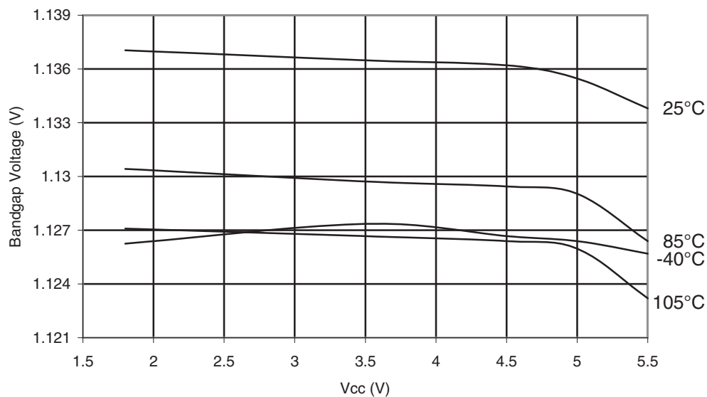
Figure 31-365. ATmega328P: Calibrated Bandgap Voltage vs. Vcc
