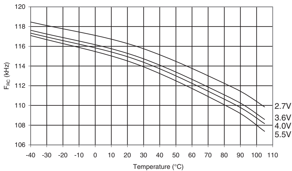
Figure 31-366. ATmega328P: Watchdog Oscillator Frequency vs. Temperature
