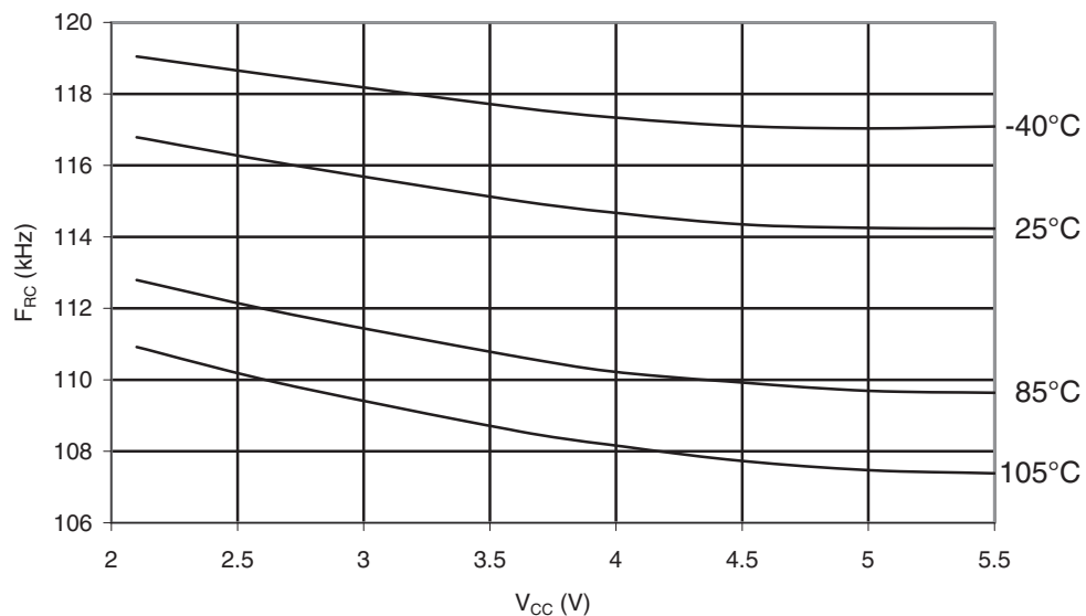
Figure 35-36. ATmega328P°C Watchdog Oscillator Frequency vs. V_{CC}
