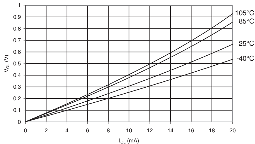
Figure 31-257. ATmega168PA: I/O Pin Output Voltage vs. Sink Current ( V_{CC} = 3V )
