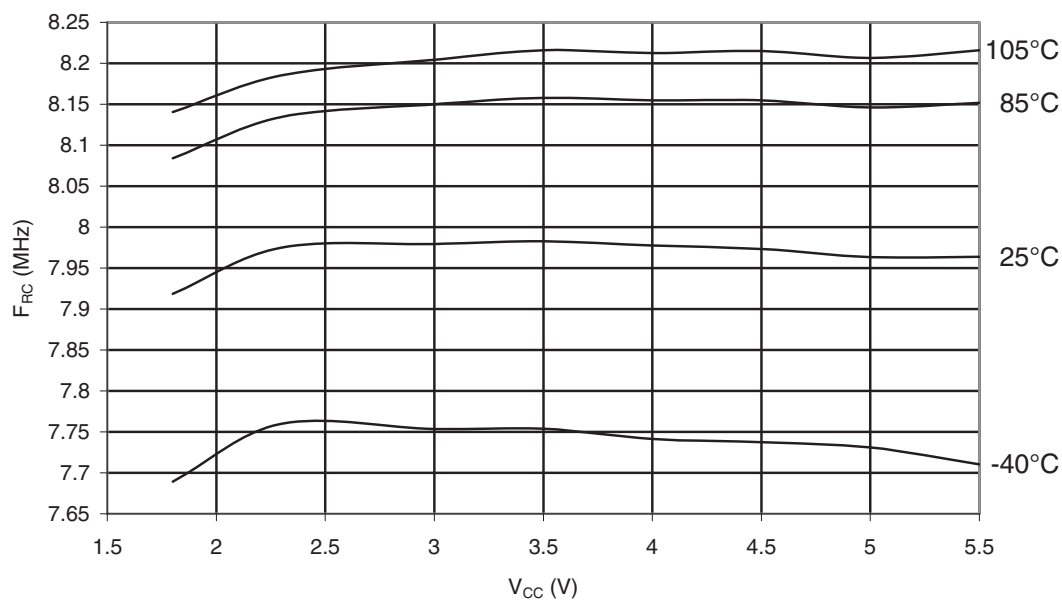
Figure 32-35. ATmega48PA: Calibrated 8MHz RC Oscillator Frequency vs. V_{CC}
