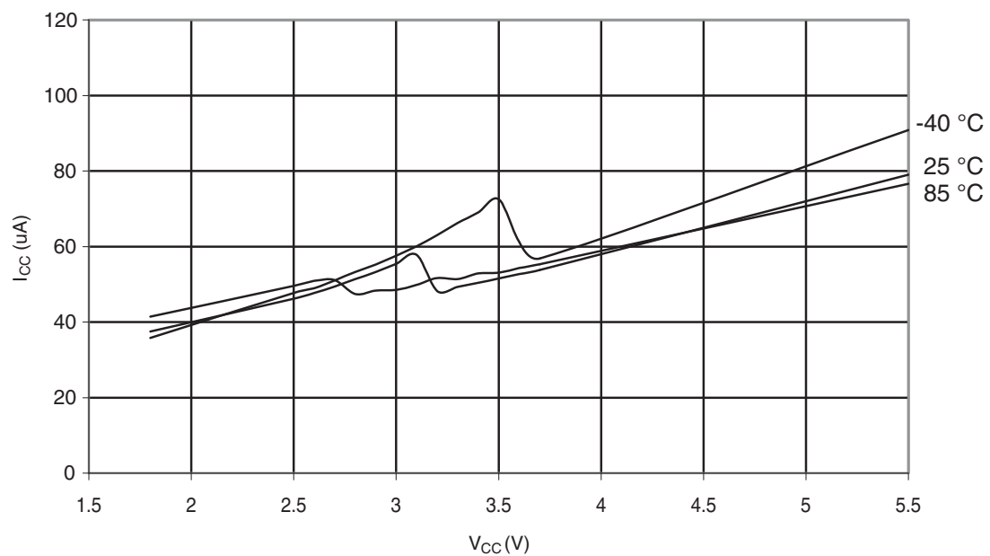
Figure 31-325. ATmega328: Analog Comparator Current vs. V_{CC}
