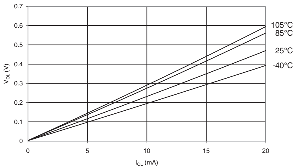
Figure 35-22. ATmega328P: I/O Pin Output Voltage vs. Sink Current ( V_{CC} = 5V )
