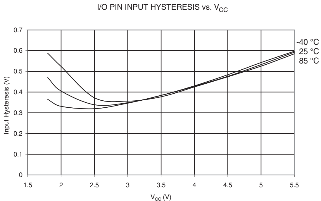
Figure 31-311. ATmega328: I/O Pin Input Hysteresis vs. V_{CC}
