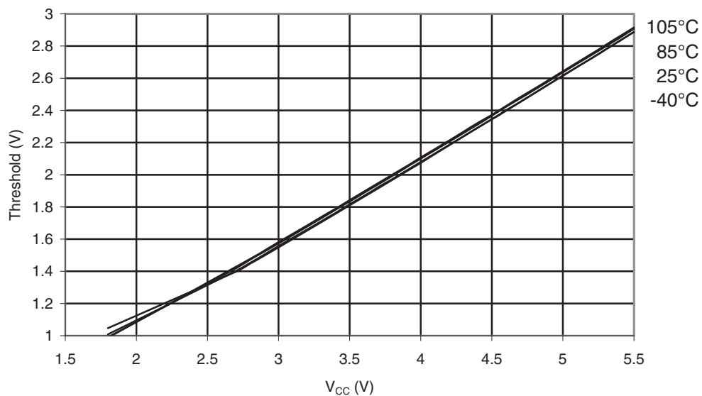
Figure 34-25. ATmega168PA I/O Pin Input Threshold Voltage vs. V_{CC} ( V_{IH} , I/O Pin read as '1')
