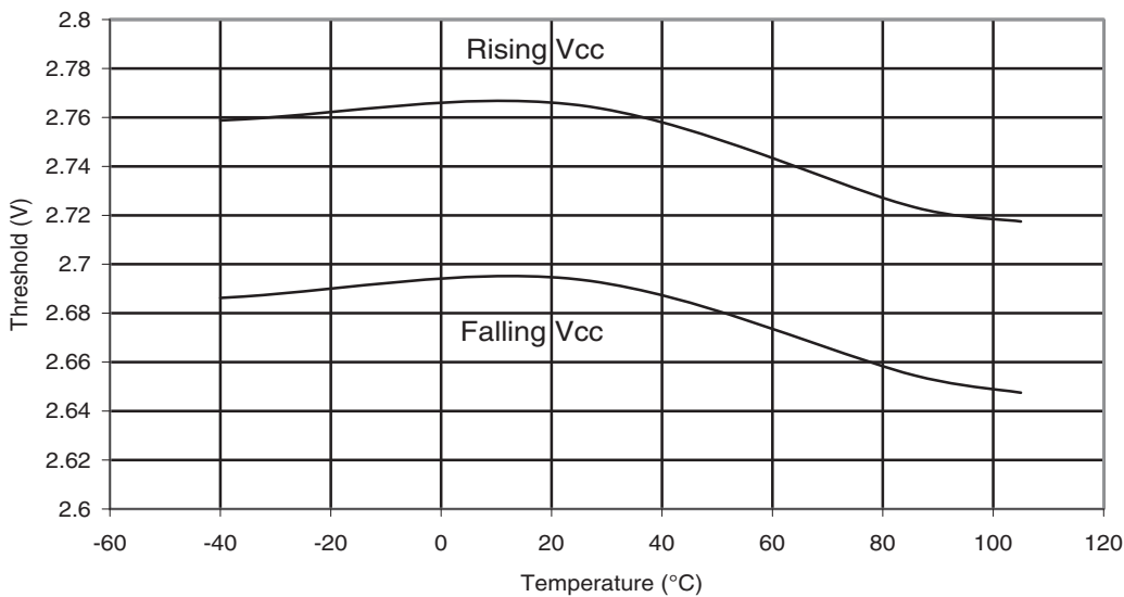
Figure 33-31.ATmega88PA: BOD Thresholds vs. Temperature (BODLEVEL is 2.7V)
