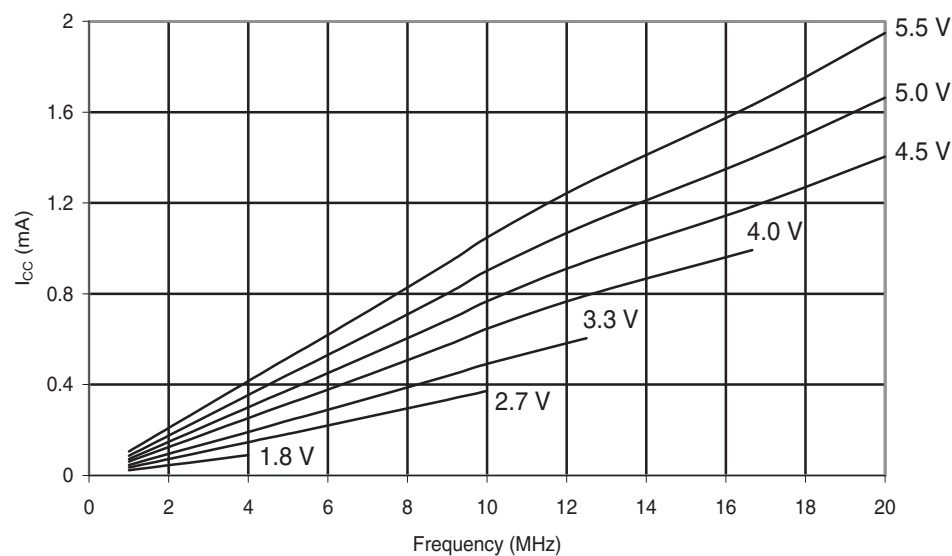
Figure 31-140. ATmega88A: Reset Supply Current vs. Frequency (1 - 20MHz)
