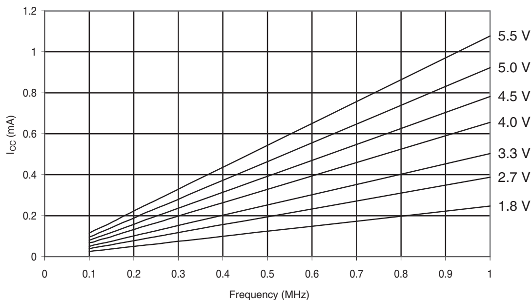
Figure 31-285. ATmega328: Active Supply Current vs. Low Frequency (0.1-1.0MHz)
