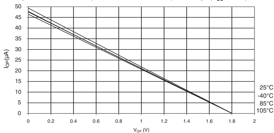
Figure 31-346. ATmega328P: I/O Pin Pull-up Resistor Current vs. Input Voltage ( V_{CC} = 1.8V )
