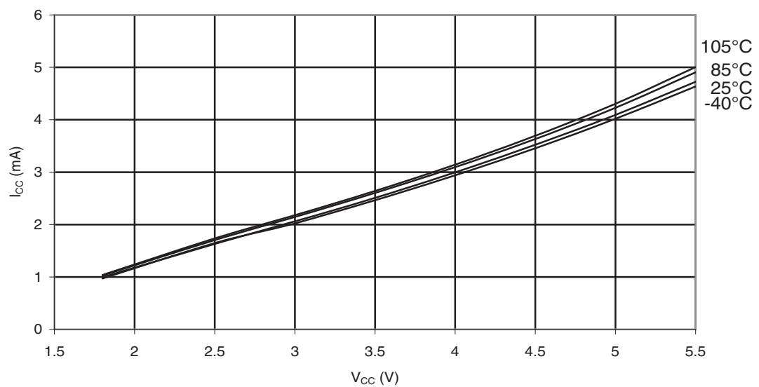
Figure 31-146. ATmega88PA: Active Supply Current vs. V_{CC} (Internal RC Oscillator, 8MHz)
