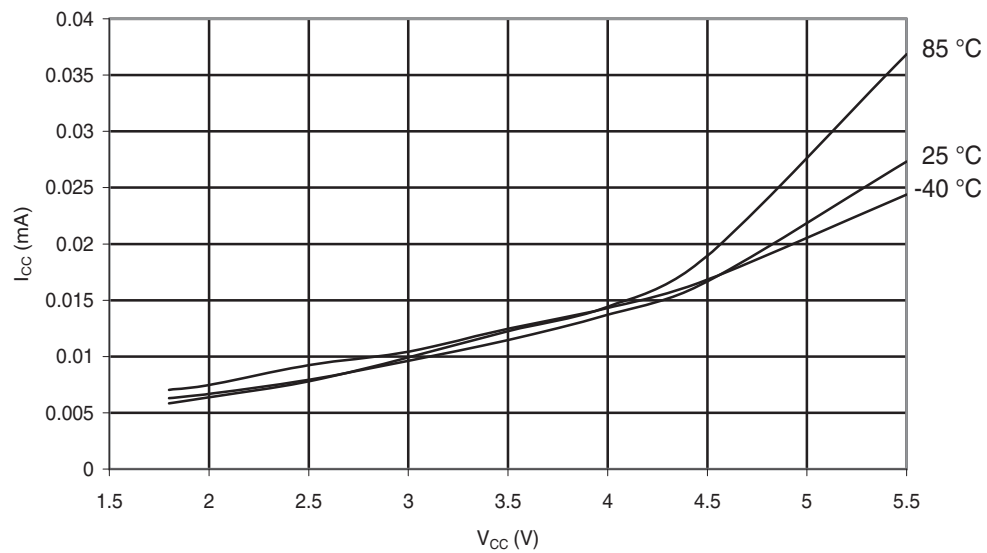
Figure 31-197. IATmega168A: Idle Supply Current vs. V_{CC} (Internal RC Oscillator, 128kHz)
