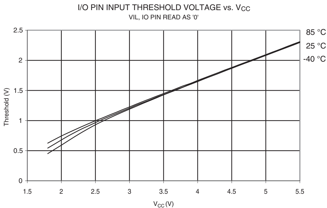
Figure 31-310. ATmega328: I/O Pin Input Threshold Voltage vs. V_{CC} ( V_{IL} , I/O Pin read as '0')
