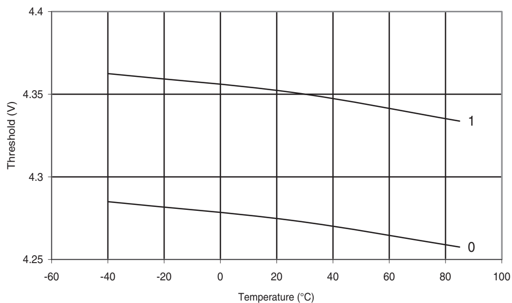
Figure 31-317. ATmega328: BOD Thresholds vs. Temperature (BODLEVEL is 4.3 V)
