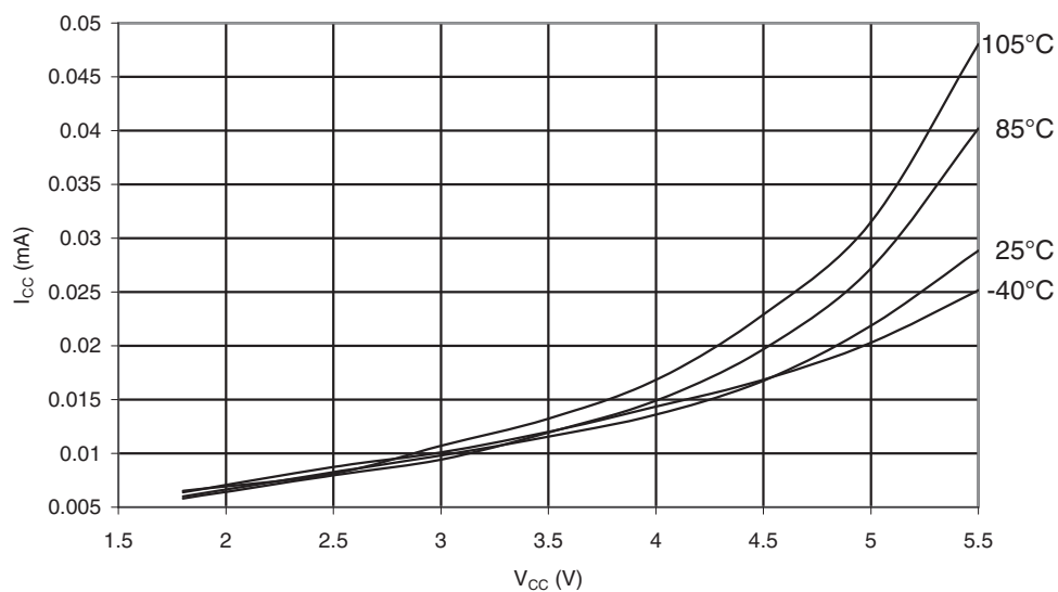
Figure 31-50. ATmega48PA: Active Supply Current vs. V_{CC} (Internal RC Oscillator, 128kHz)
