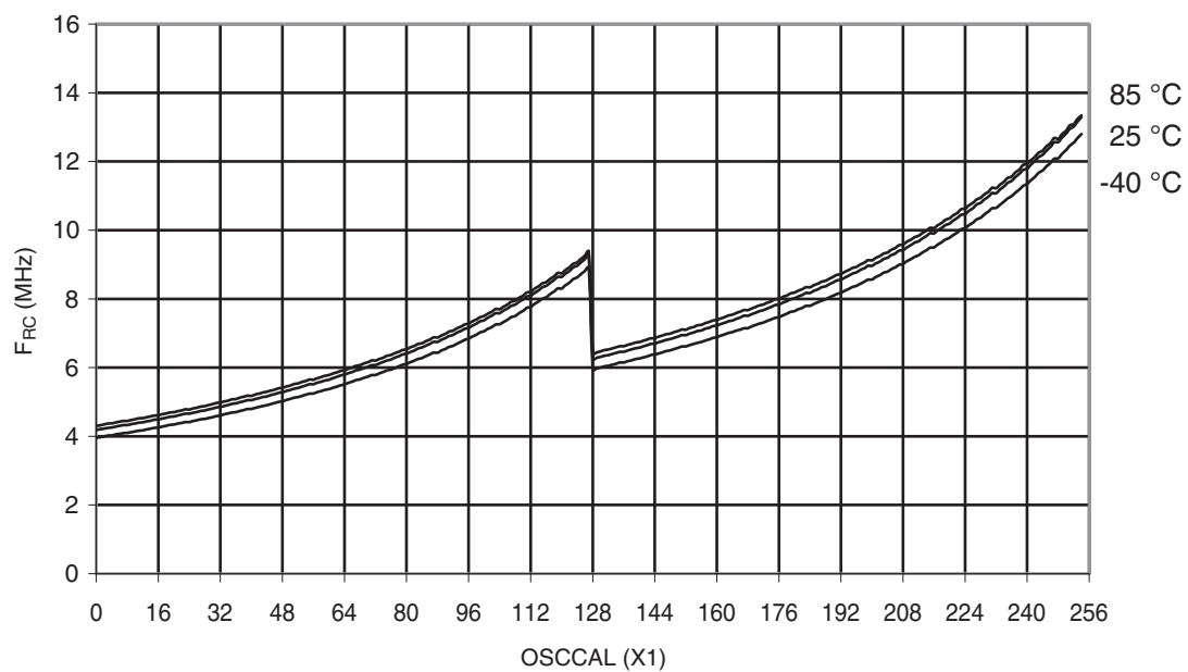
Figure 31-323. ATmega328: Calibrated 8MHz RC Oscillator Frequency vs. OSCCAL Value
