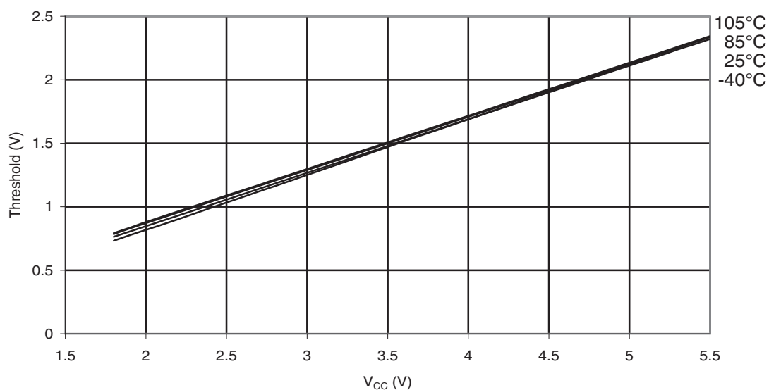
Figure 31-170. ATmega88PA: Reset Input Threshold Voltage vs. V_{CC} ( V_{IL} , I/O Pin read as '0')
