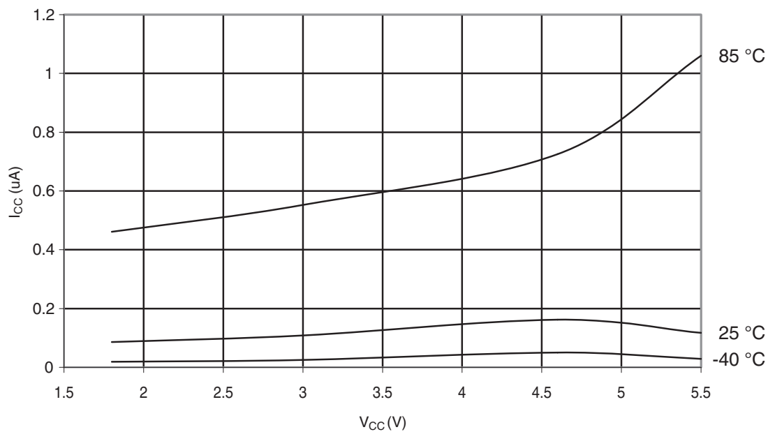
Figure 31-295. ATmega328: Power-Down Supply Current vs. V_{CC} (Watchdog Timer Disabled)
