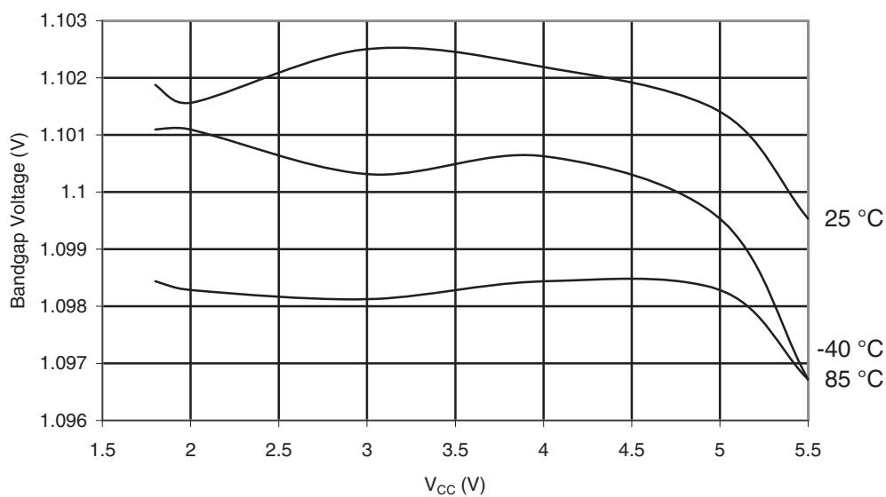
Figure 31-128. ATmega88A: Bandgap Voltage vs. V_{CC}
