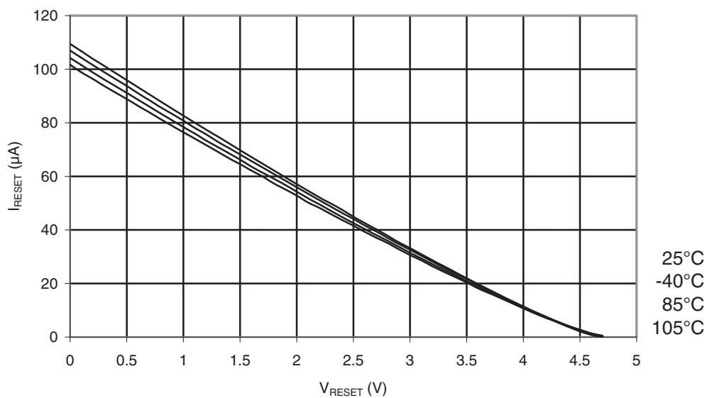
Figure 31-256. ATmega168PA: Reset Pull-up Resistor Current vs. Reset Pin Voltage ( V_{CC} = 5V )
