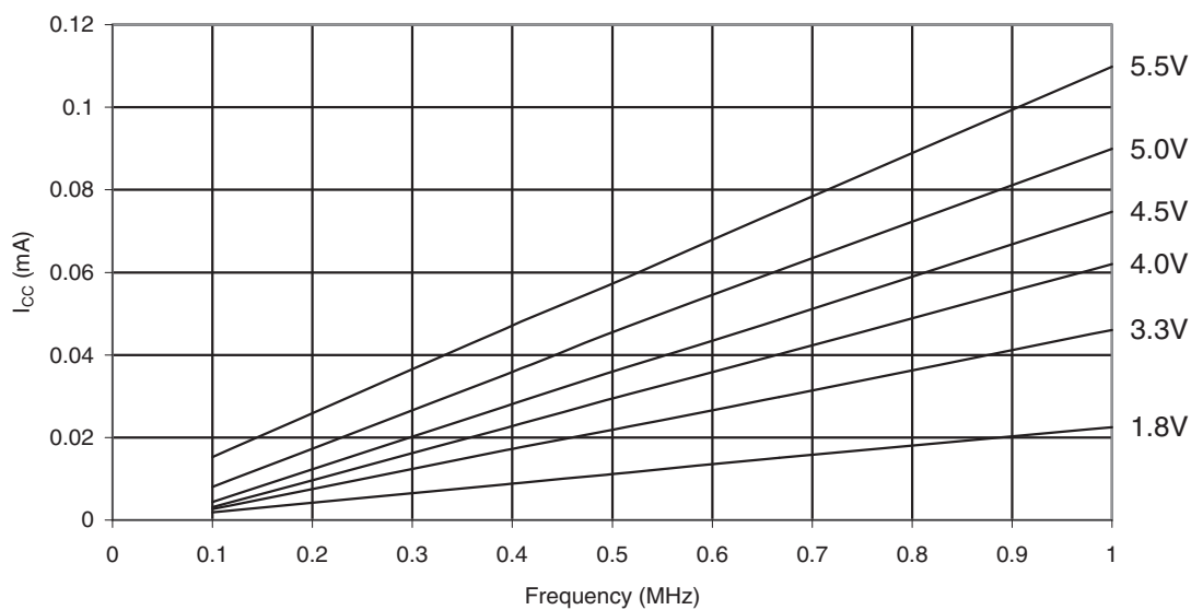
Figure 33-43. ATmega88PA: Reset Supply Current vs. Low Frequency (0.1MHz - 1.0MHz)
