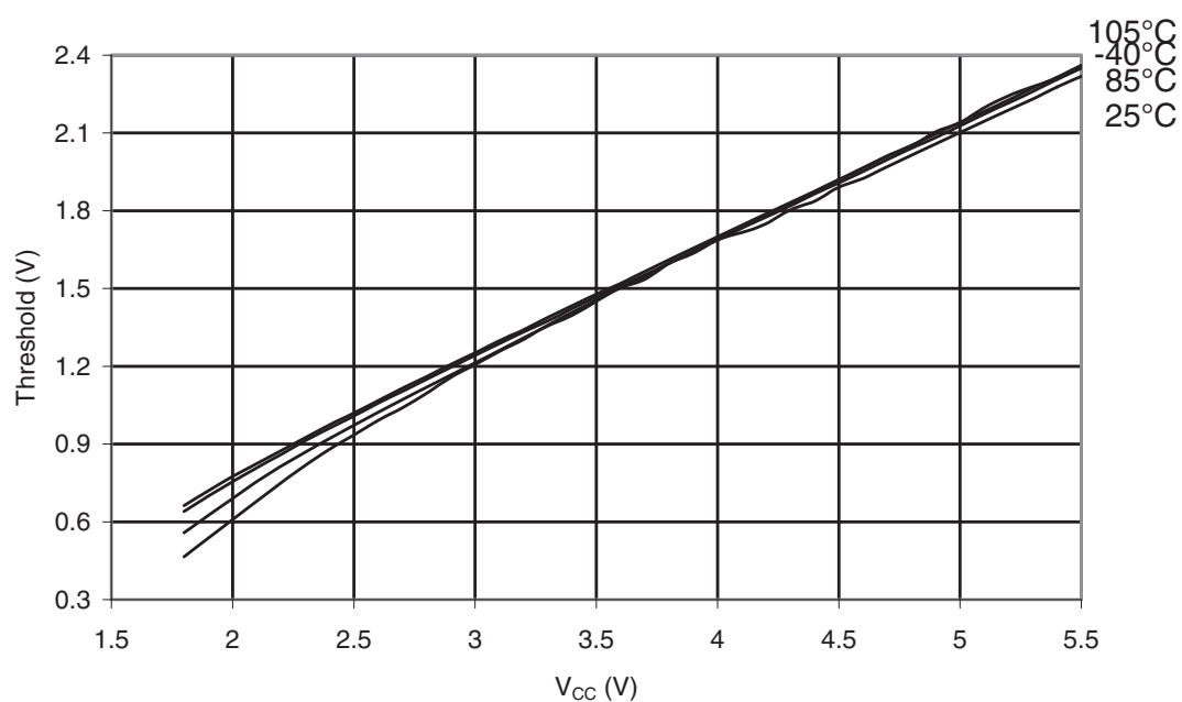
Figure 31-73. ATmega48PA: I/O Pin Input Threshold Voltage vs. V_{CC} ( V_{IL} , I/O Pin read as '0')
