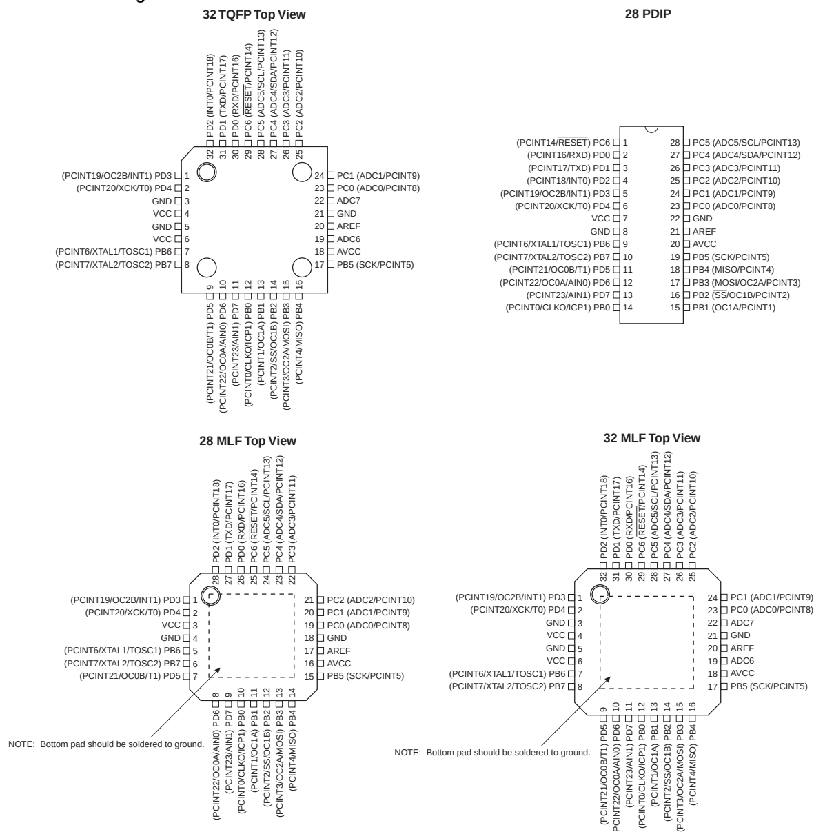
Figure 1-1. Pinout ATmega48A/PA/88A/PA/168A/PA/328/P
