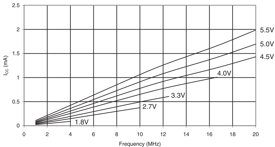
Figure 33-44. ATmega88PA: Reset Supply Current vs. Frequency (1MHz - 20MHz)
