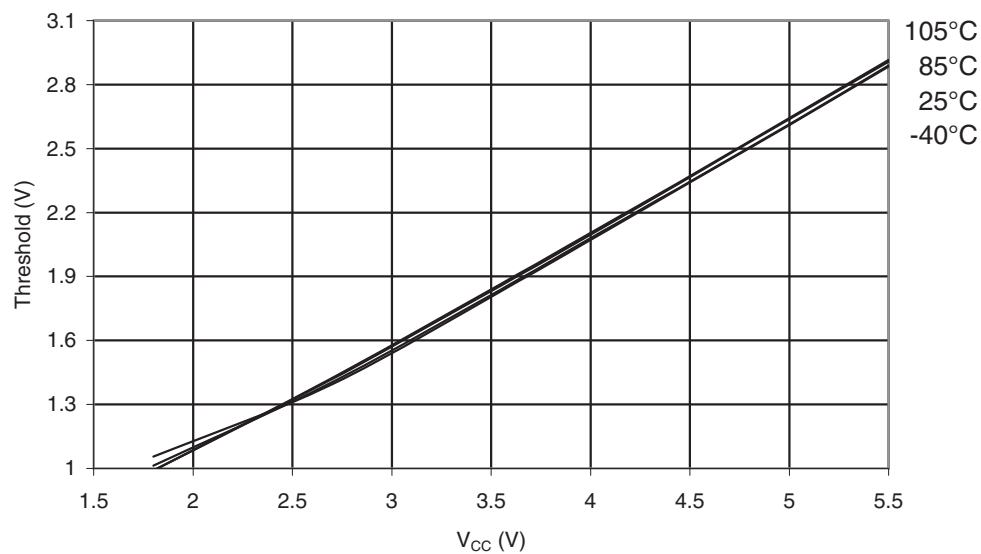
Figure 35-25. ATmega328P: I/O Pin Input Threshold Voltage vs. V_{CC} ( V_{IH} , I/O Pin read as '1')
