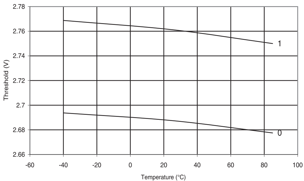
Figure 31-316. ATmega328: BOD Thresholds vs. Temperature (BODLEVEL is 2.7 V)
