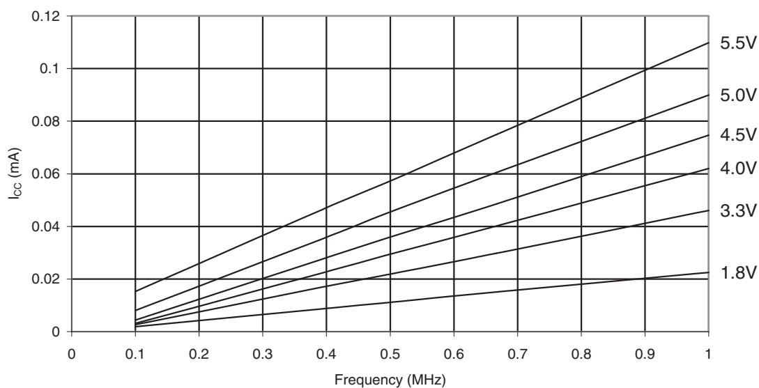
Figure 31-187. ATmega88PA: Reset Supply Current vs. Low Frequency (0.1MHz - 1.0MHz)
