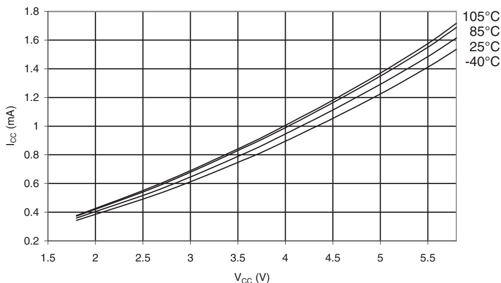
Figure 31-341. ATmega328P Idle Supply Current vs. V CC (Internal RC Oscillator, 8MHz)
