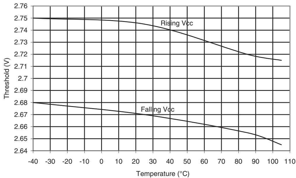
Figure 32-31.ATmega48PA: BOD Thresholds vs. Temperature (BODLEVEL is 2.7V)
