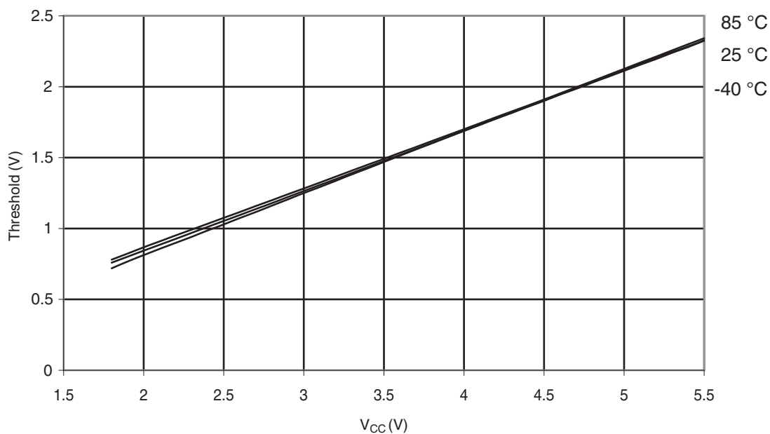
Figure 31-313. ATmega328: Reset Input Threshold Voltage vs. V_{CC} ( V_{IL} , I/O Pin read as '0')
