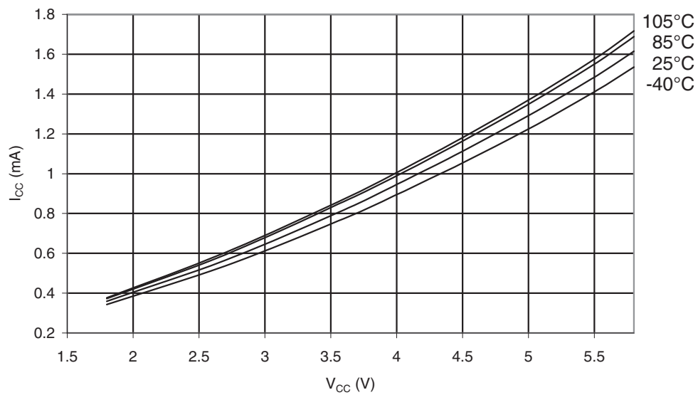
Figure 35-10. ATmega328P Idle Supply Current vs. V_{CC} (Internal RC Oscillator, 8MHz)
