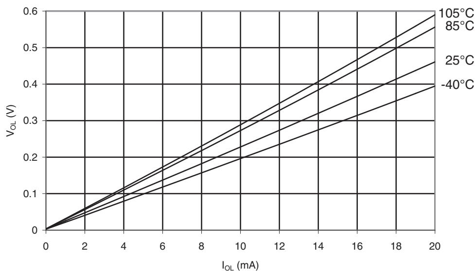
Figure 34-22. ATmega168PA: I/O Pin Output Voltage vs. Sink Current ( V_{CC} = 5V )
