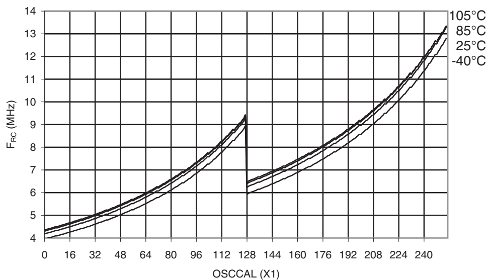
Figure 35-39. ATmega328P Calibrated 8MHz RC Oscillator Frequency vs. OSCAL Value
