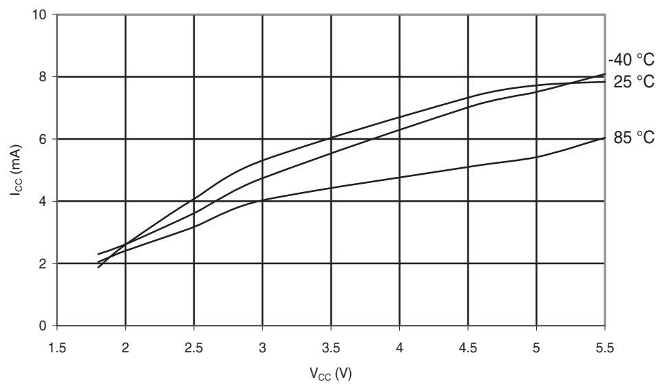
Figure 31-233. ATmega168A: Programming Current vs. V_{CC}
