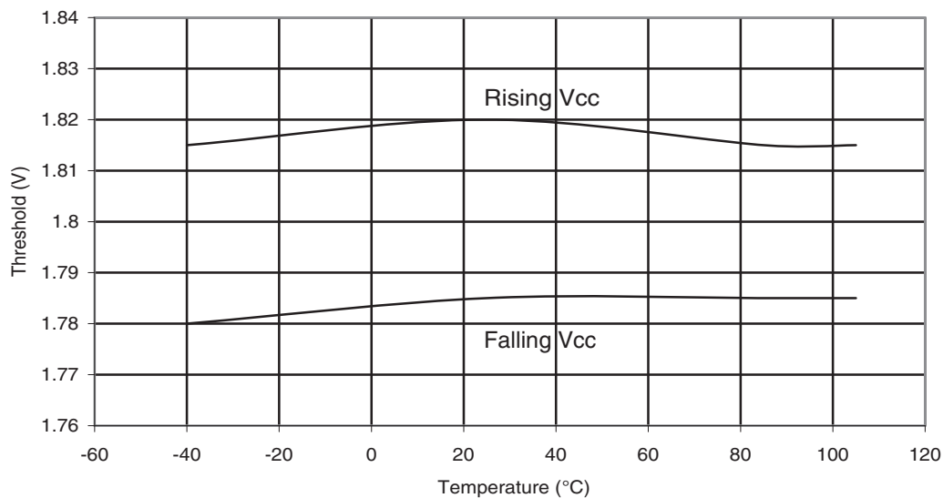
Figure 33-30.ATmega88PA: BOD Thresholds vs. Temperature (BODLEVEL is 1.8V)
