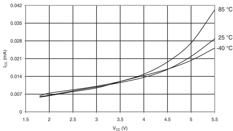
Figure 31-8. ATmega48A: Idle Supply Current vs. V_{CC} (Internal RC Oscillator, 128kHz)
