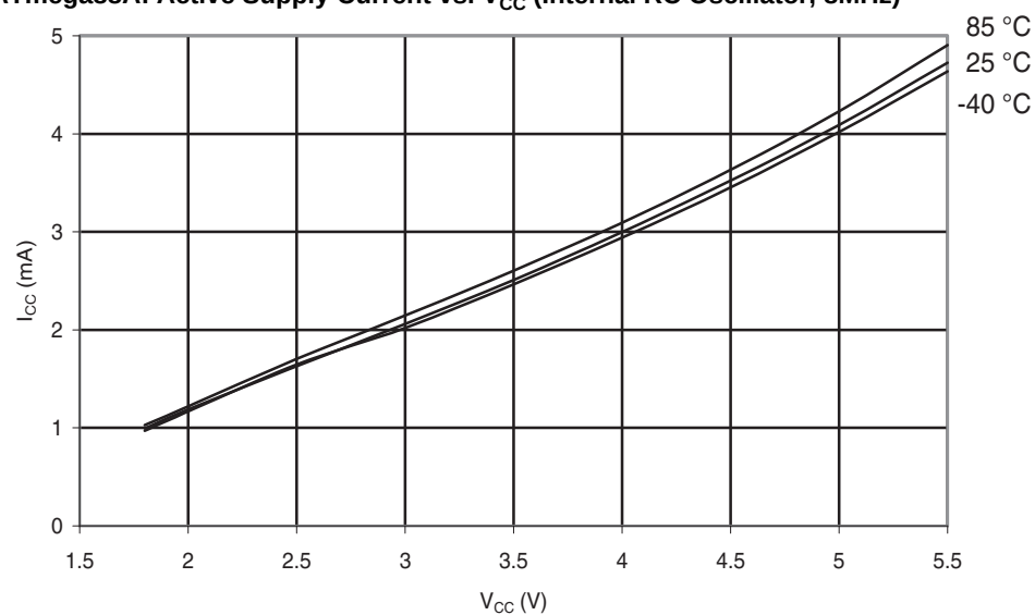
Figure 31-99. ATmega88A: Active Supply Current vs. V_{CC} (Internal RC Oscillator, 8MHz)
