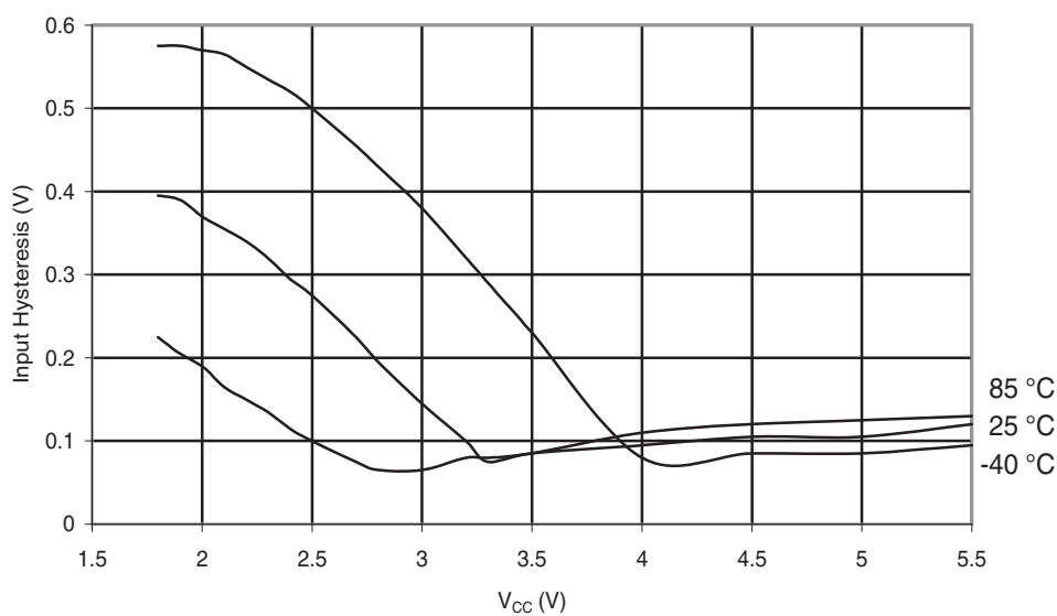
Figure 31-124. ATmega88A: Reset Pin Input Hysteresis vs. V_{CC}
