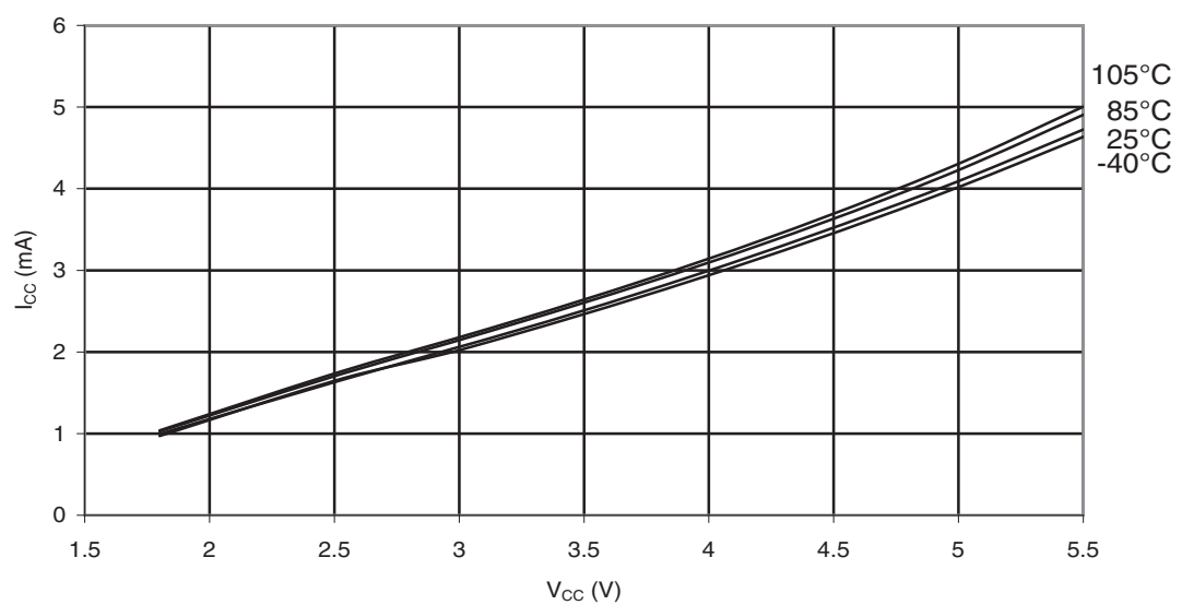
Figure 33-5. ATmega88PA: Active Supply Current vs. V_{CC} (Internal RC Oscillator, 8MHz)
