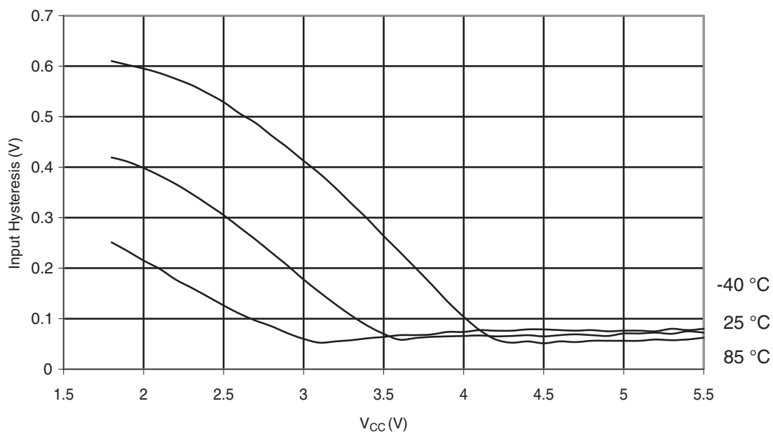
Figure 31-314. ATmega328: Reset Pin Input Hysteresis vs. V_{CC}
