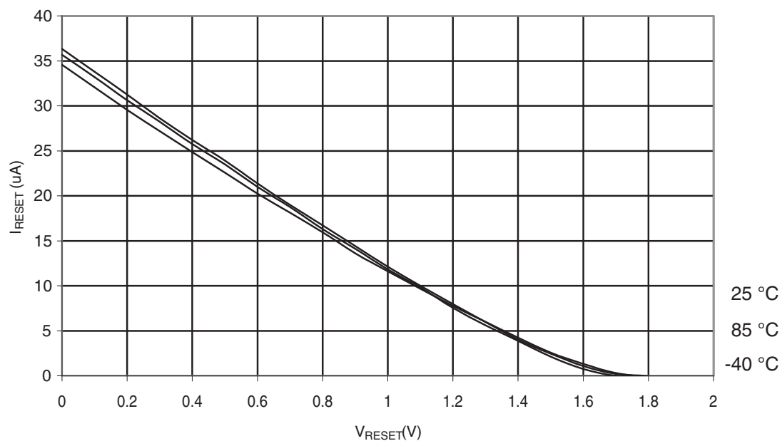
Figure 31-302. ATmega328: Reset Pull-up Resistor Current vs. Reset Pin Voltage ( V_{CC} = 1.8\text{ V} )
