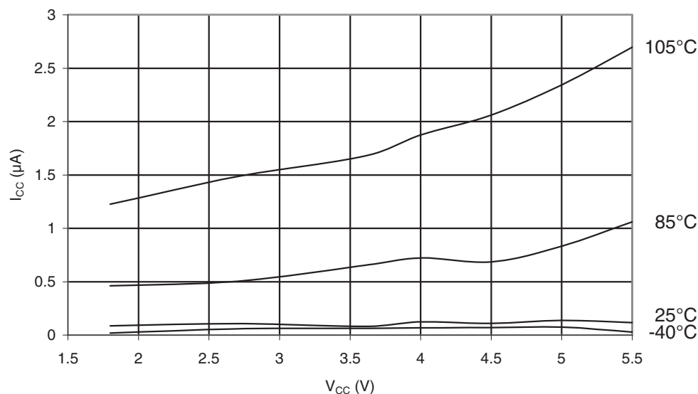
Figure 31-342. ATmega328P: Power-Down Supply Current vs. V_{CC} (Watchdog Timer Disabled)
