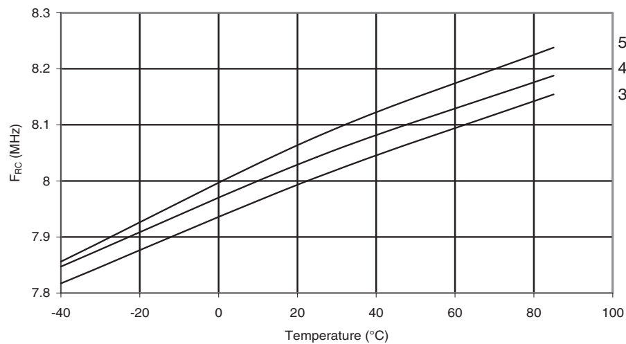
Figure 31-132. ATmega88A: Calibrated 8MHz RC Oscillator Frequency vs. Temperature
