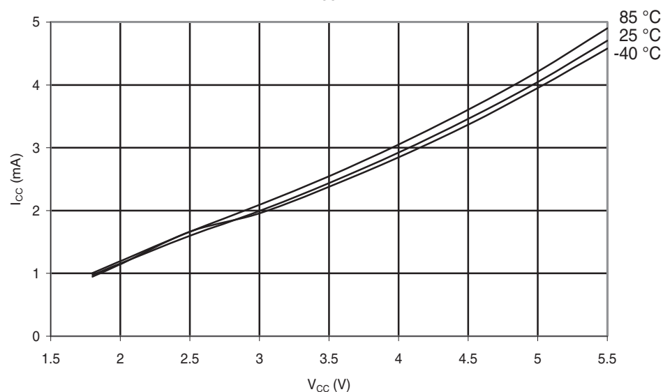
Figure 31-5. ATmega48A: Active Supply Current vs. V_{CC} (Internal RC Oscillator, 8MHz)
