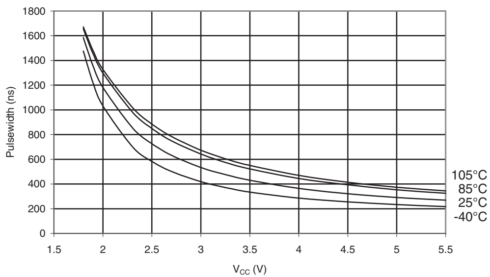
Figure 34-48. ATmega168PA: Minimum Reset Pulse Width vs. V CC
