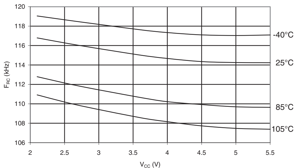
Figure 31-367. ATmega328P°C Watchdog Oscillator Frequency vs. V_{CC}
