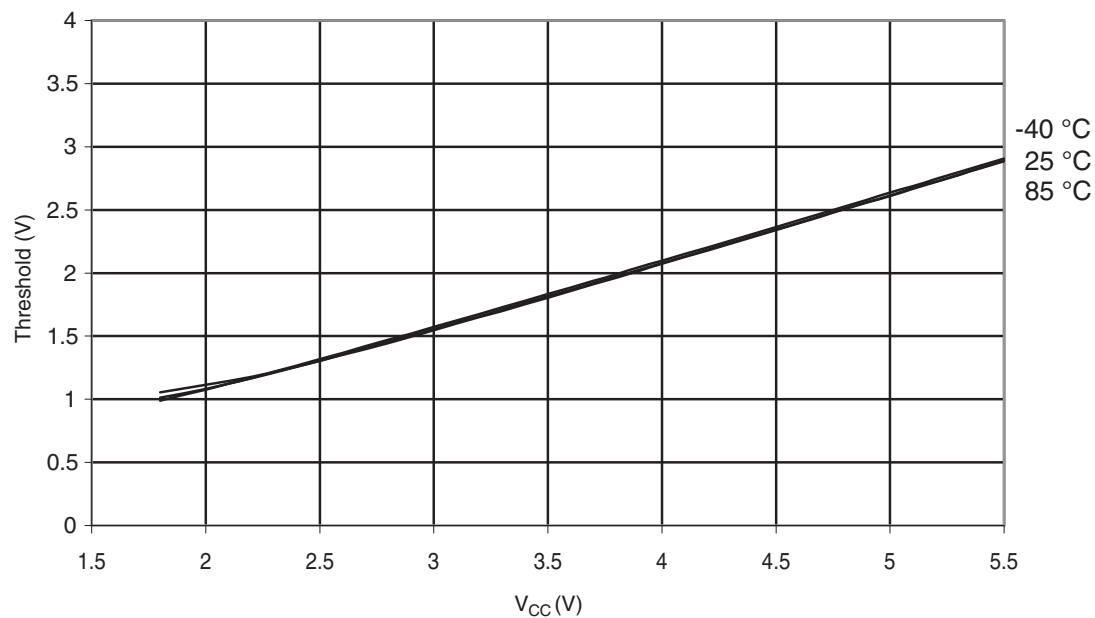
Figure 31-309. ATmega328: I/O Pin Input Threshold Voltage vs. V_{CC} ( V_{IH} , I/O Pin read as '1')
