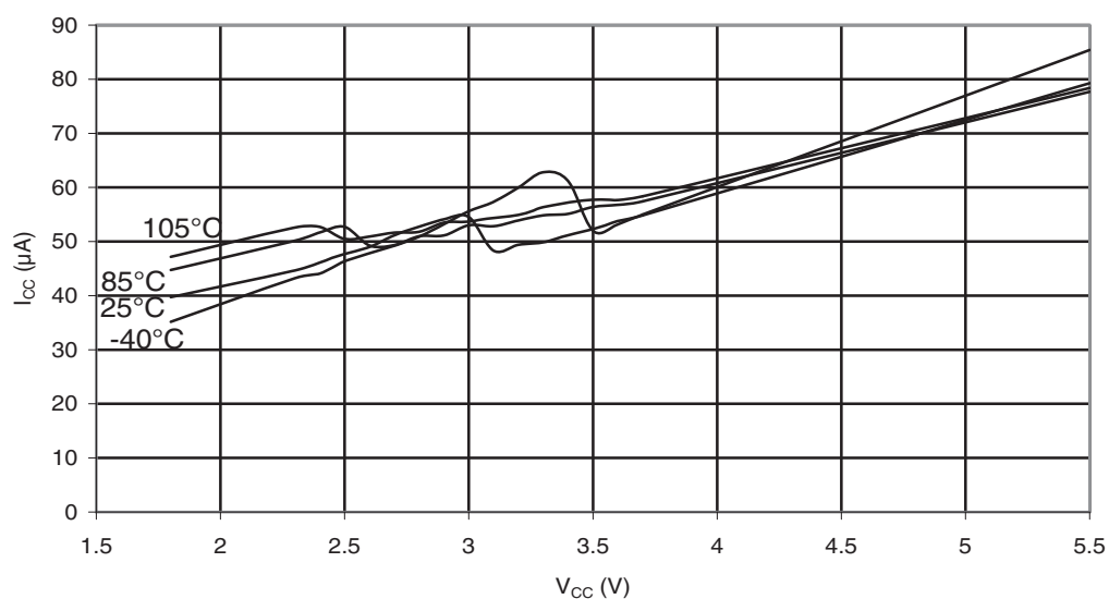
Figure 33-39. ATmega88PA: Analog Comparator Current vs. V_{CC}
