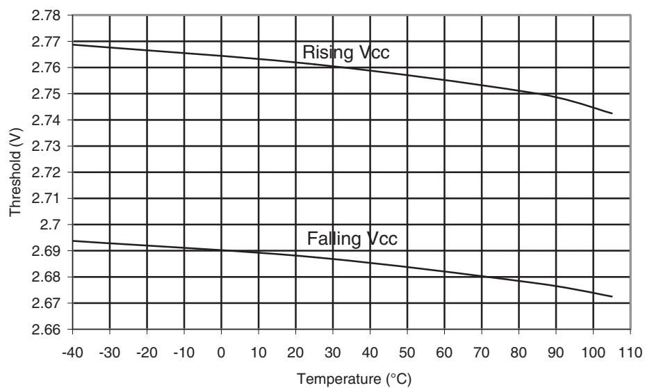
Figure 31-363. ATmega328P BOD Thresholds vs. Temperature (BODLEVEL is 2.7V)
