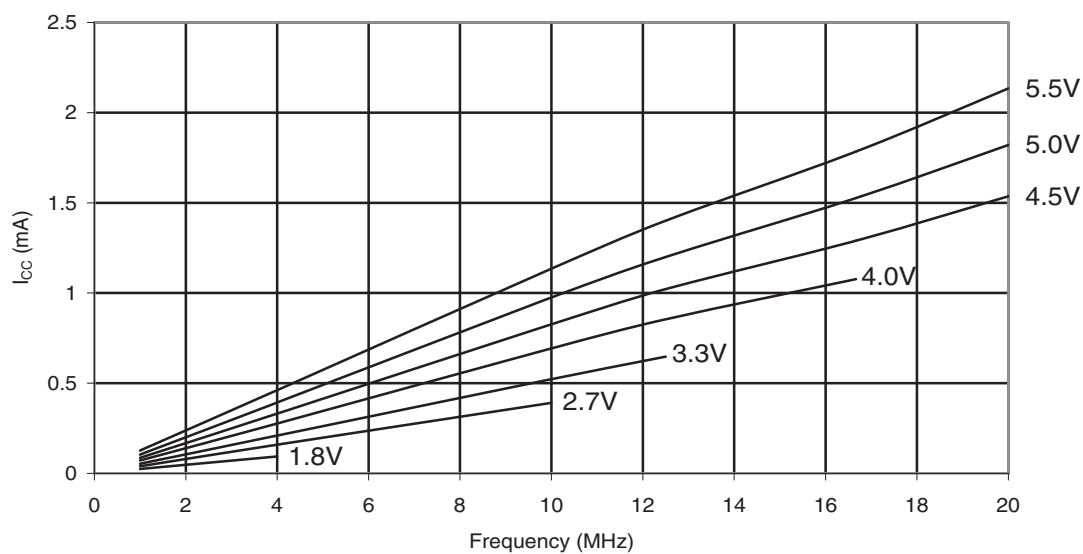
Figure 33-7. ATmega88PA: Idle Supply Current vs. Frequency (1MHz - 20MHz)
