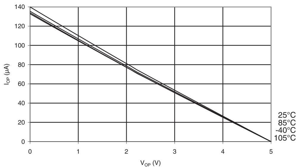
Figure 34-17. ATmega168PA: I/O Pin Pull-up Resistor Current vs. Input Voltage ( V_{CC} = 5V )
