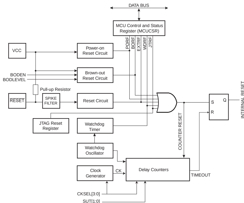
Figure 15. Reset Logic
