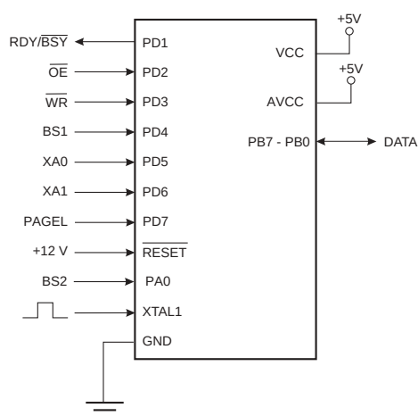
Figure 127. Parallel Programming
