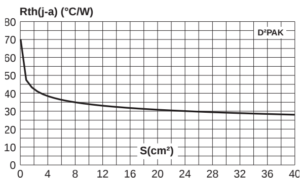
Fig. 10: D 2 PAK Thermal resistance junction to ambient versus copper surface under tab (printed circuit board FR4, copper thickness: 35\text{ }\mu\text{m} ).
