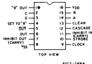
TERMINAL ASSIGNMENT
